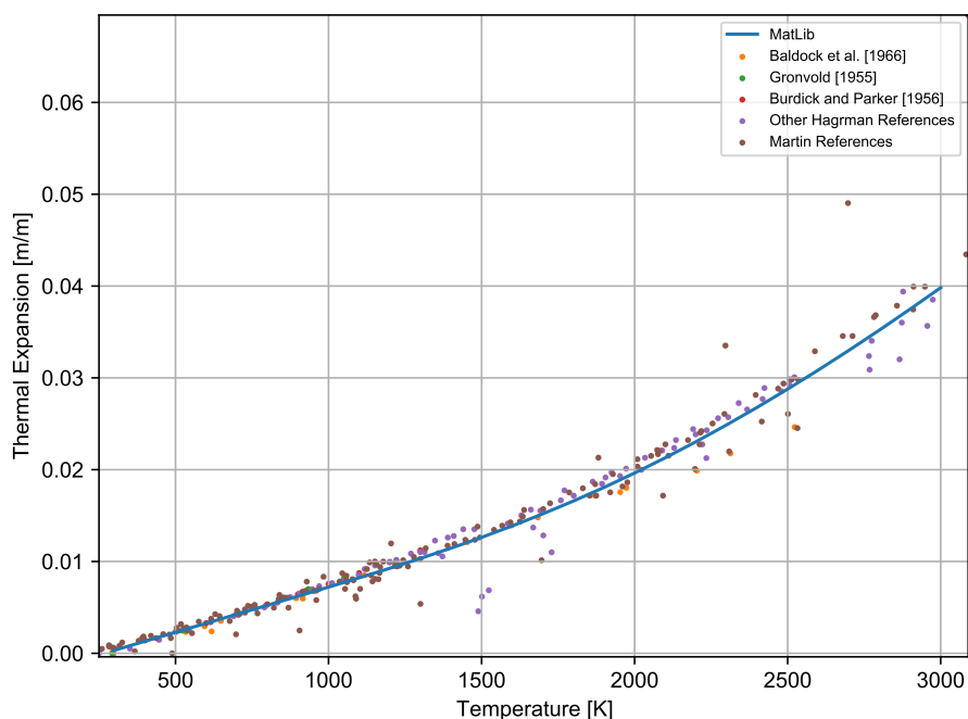
Figure 2-9. Model-to-Data Comparison for UO 2 Correlation
