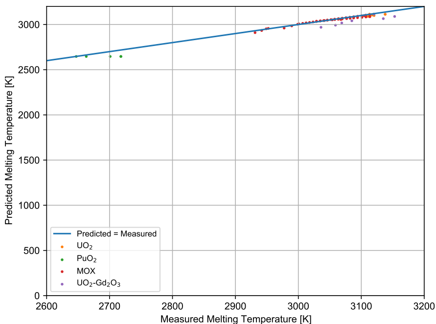
Figure 2-8. Model-to-Data Comparison for UO 2 , PuO 2 , MOX, and UO 2 -Gd 2 O 3 Melting Temperature Correlation
