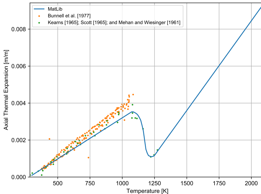
Figure 3-4. Model-to-Data Comparison for for Zirconium-based Alloy Cladding Axial Thermal Expansion Correlation
